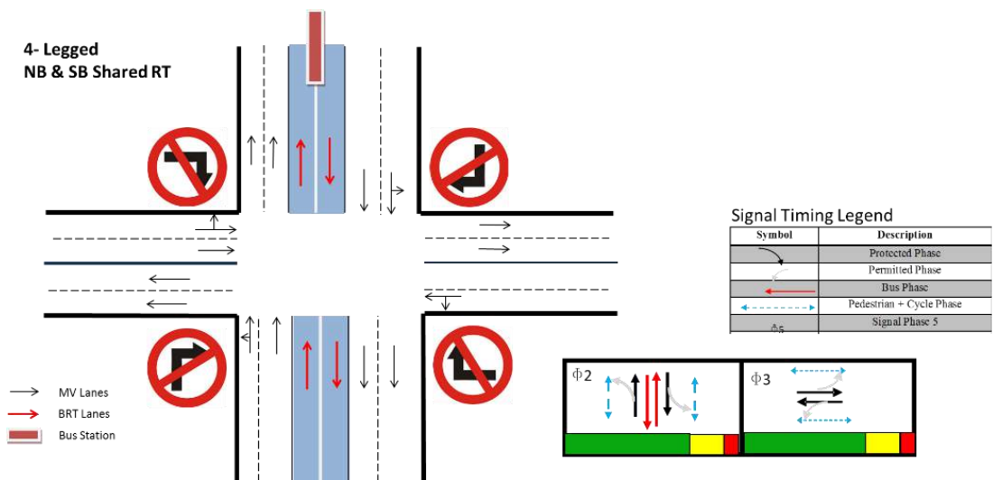
Exhibit 72: Alternative phasing option for the 4-legged intersection (with shared lanes) with BRT after turn restriction (on main and minor street) treatment
