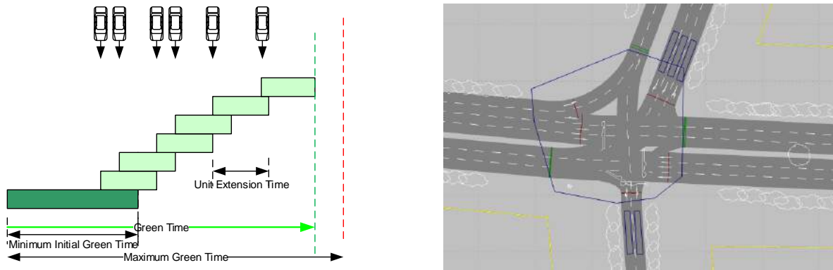
Exhibit 52: Detection for Intersection Movements - Illustration
