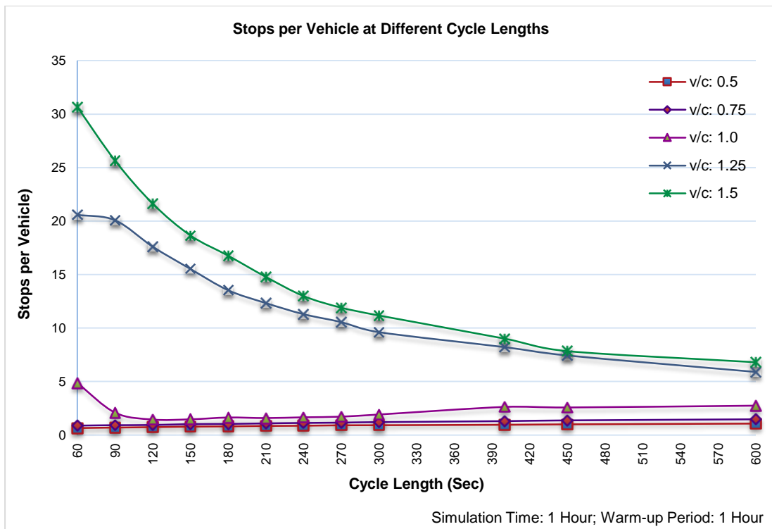
Exhibit 33: Number of Stops per Vehicle
