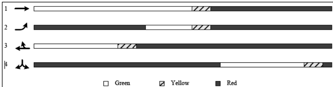
Exhibit 5: Signal Group Illustration 4
