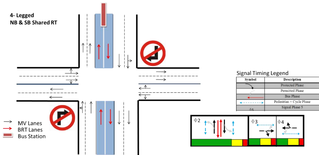
Exhibit 70: Alternative phasing option for the 4-legged intersection (with shared lanes) with BRT after turn restriction (on main street) treatment
