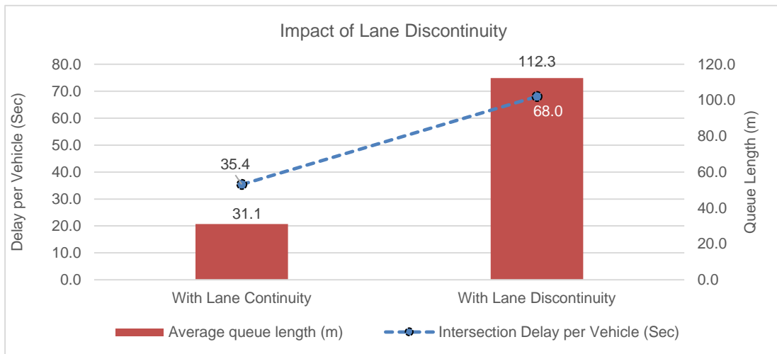
Exhibit 67: Impact of lane discontinuity on intersection delay
