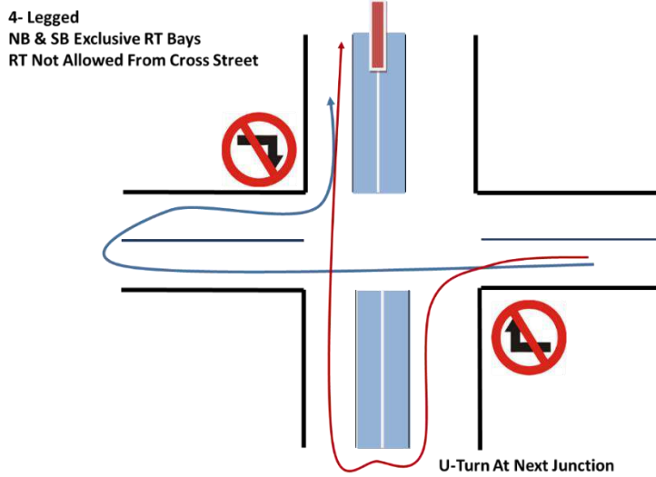
Exhibit 74: Turn restriction (on main street) treatment for the 4-legged intersection (with exclusive RT lanes) with BRT
