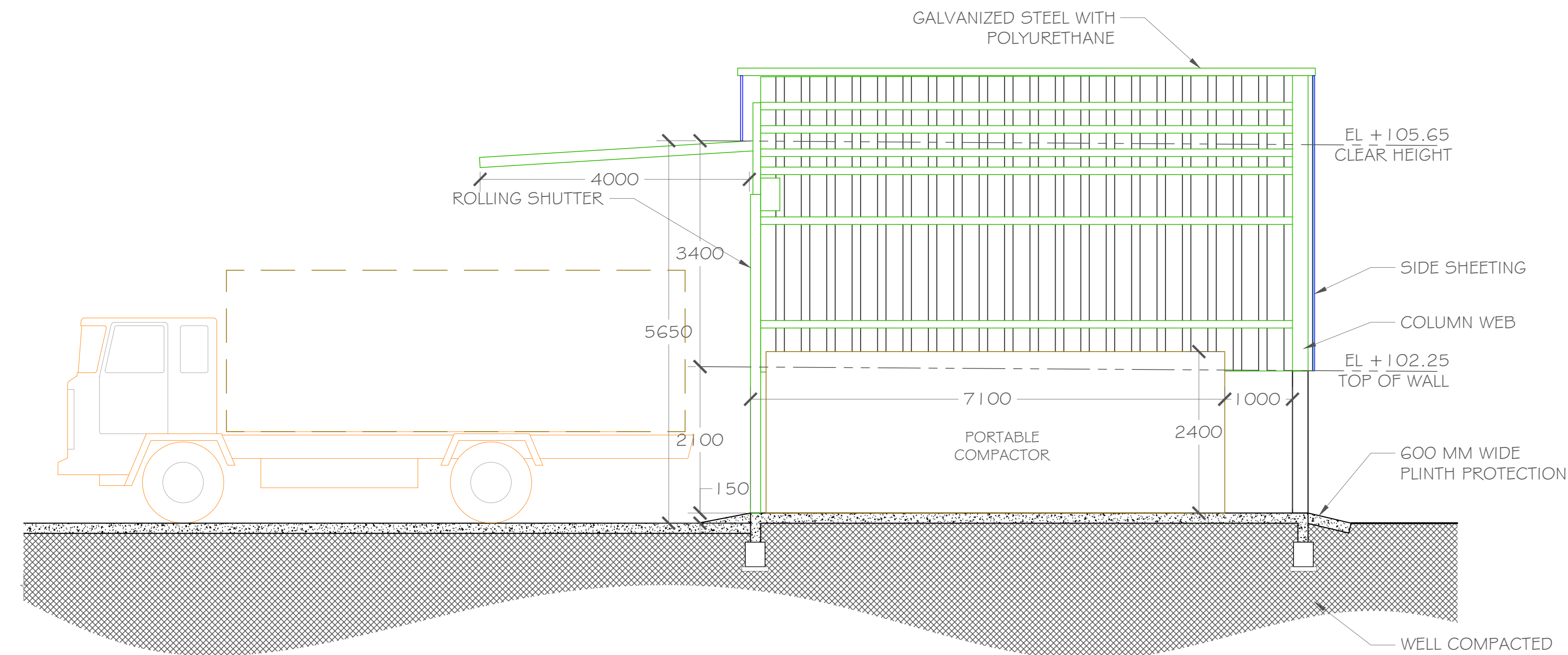
SECTION BB'
