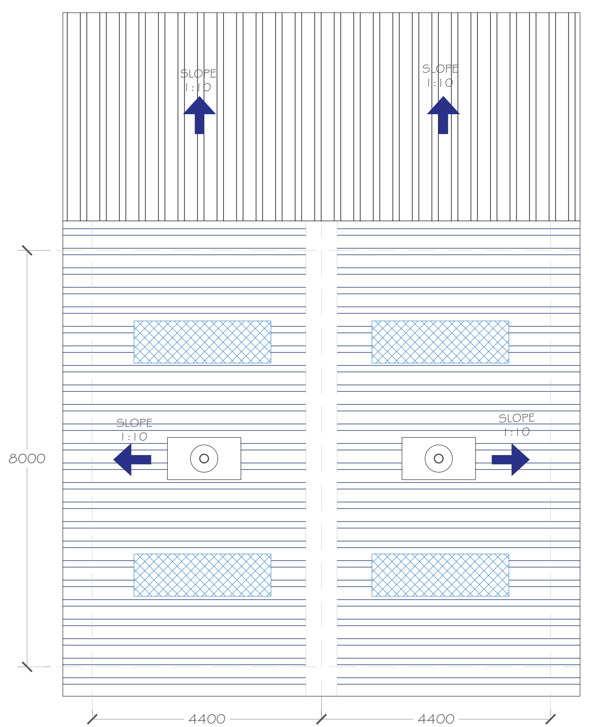
ROOF PLAN
