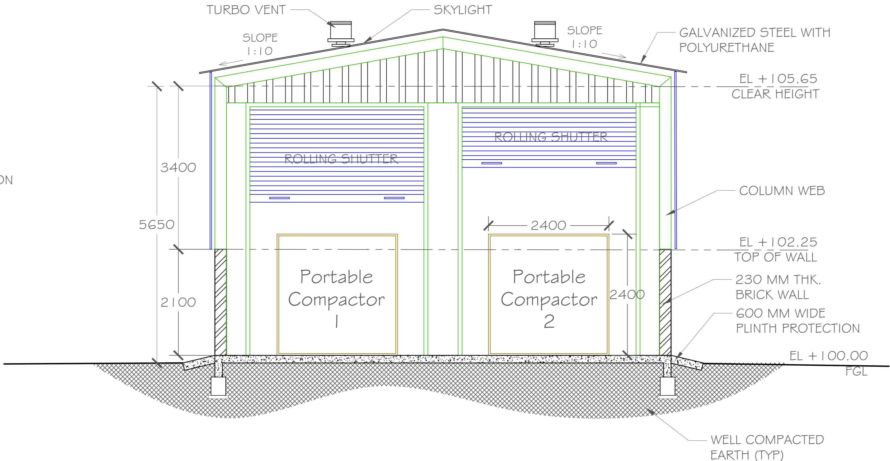
SECTION AA'
