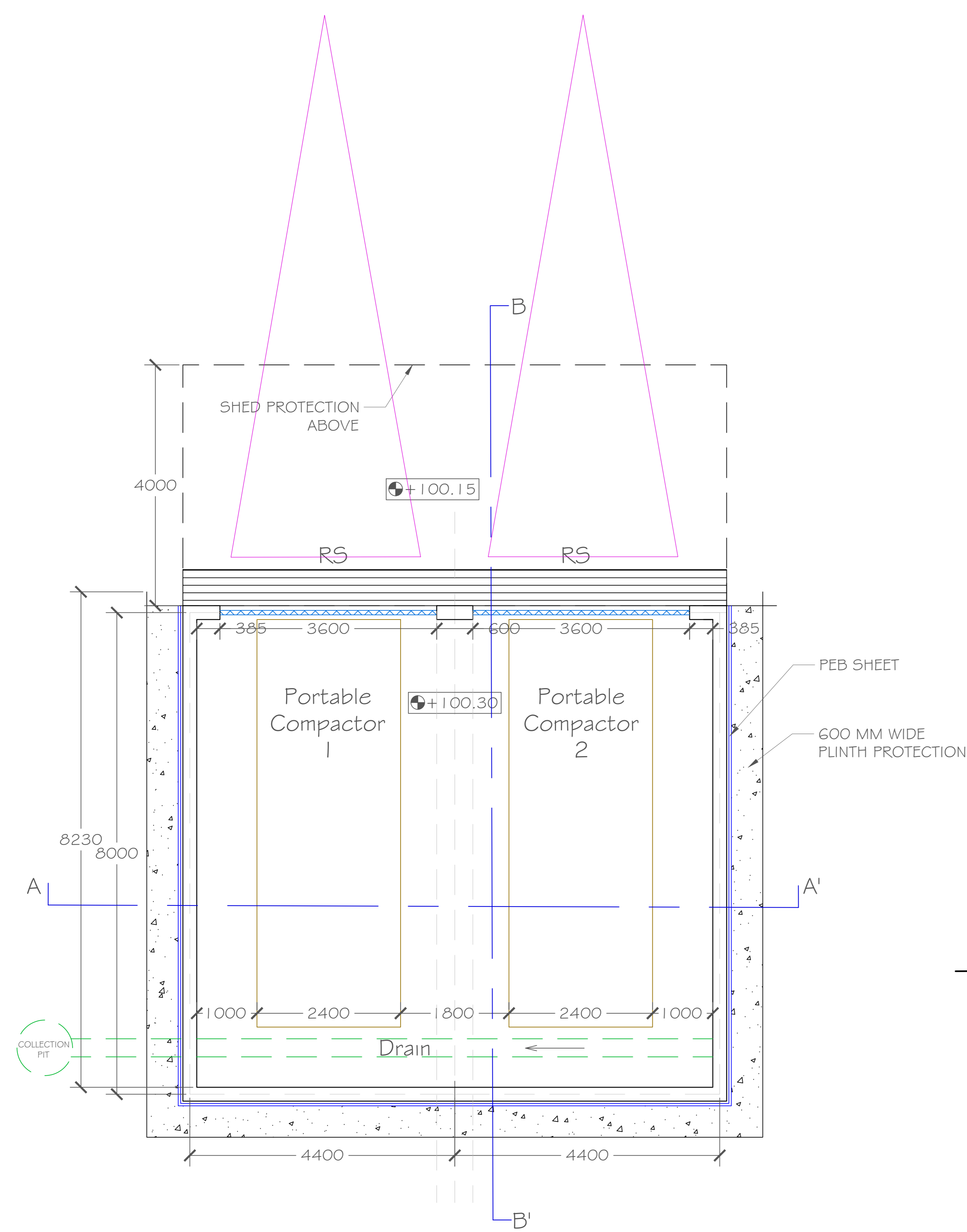
PLAN - GROUND FLOOR
