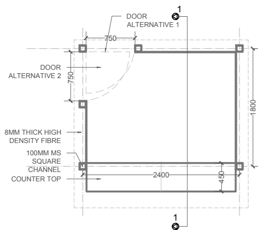
PLAN (TYP. - A) Scale-1:50
