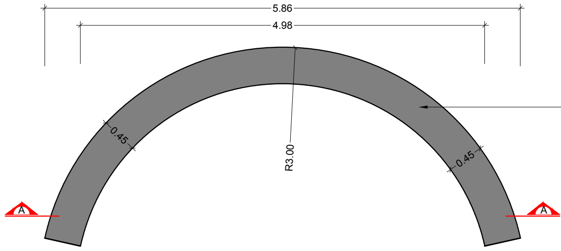
ENLARGE PLAN OF SEATING TYPE -1 (TYP.) (SCALE : 1:50)
