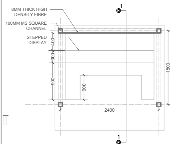
PLAN (TYP. - B) Scale-1:50
