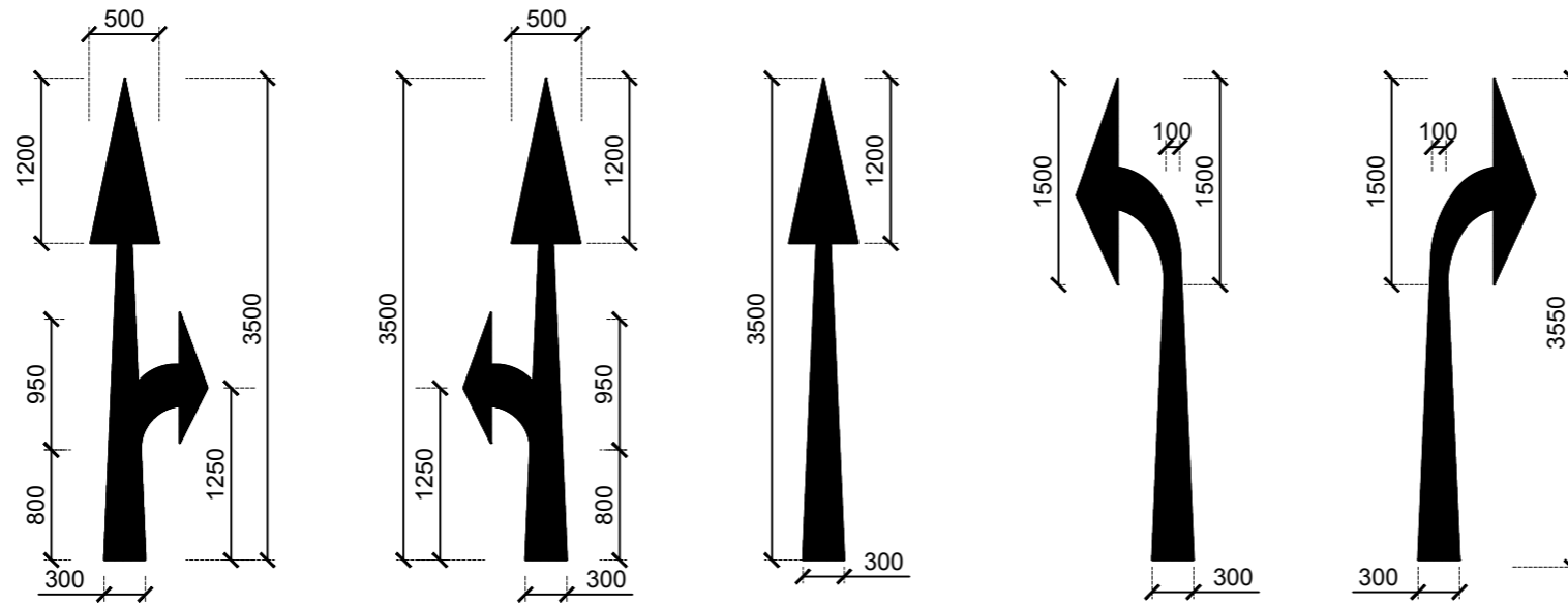
DIRECTION MARKING DETAILS 1:50
