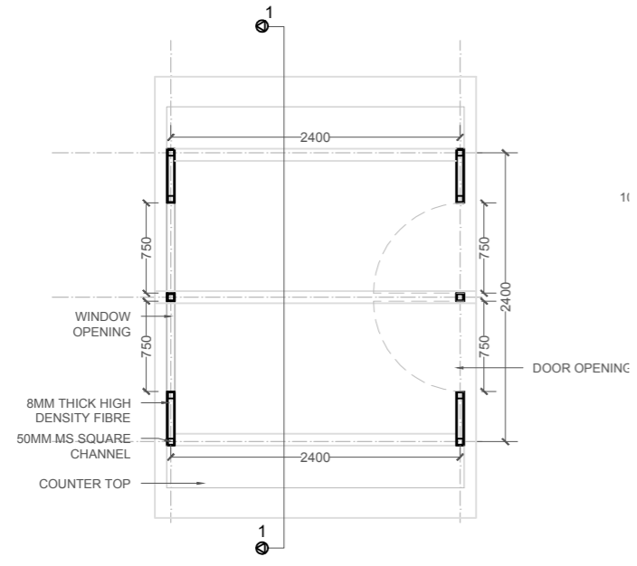
PLAN (TYP. - C) Scale-1:50
