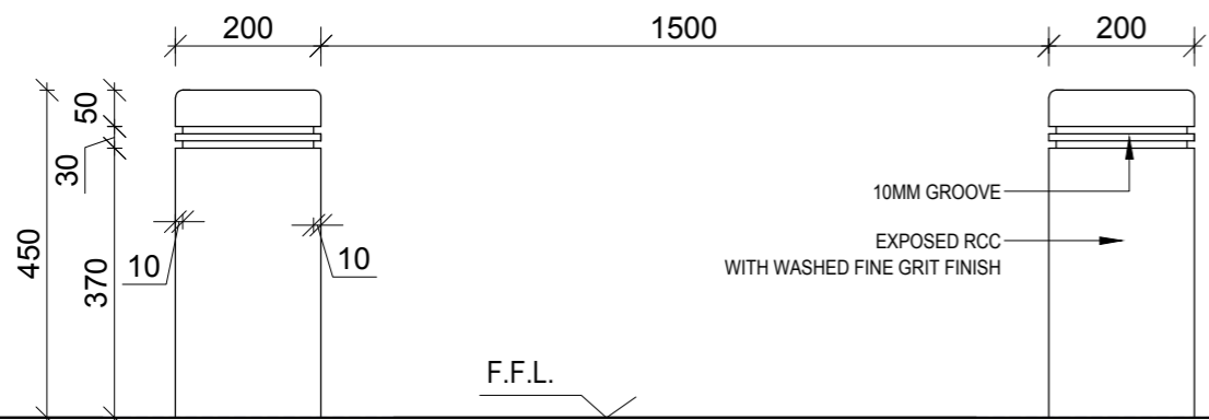
ELEVATION SCALE 1:10
