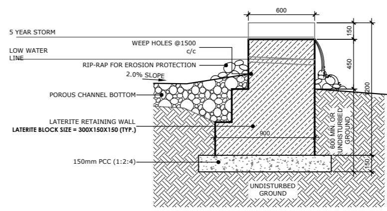
LATERITE WALL DETAIL SCALE 1:30
