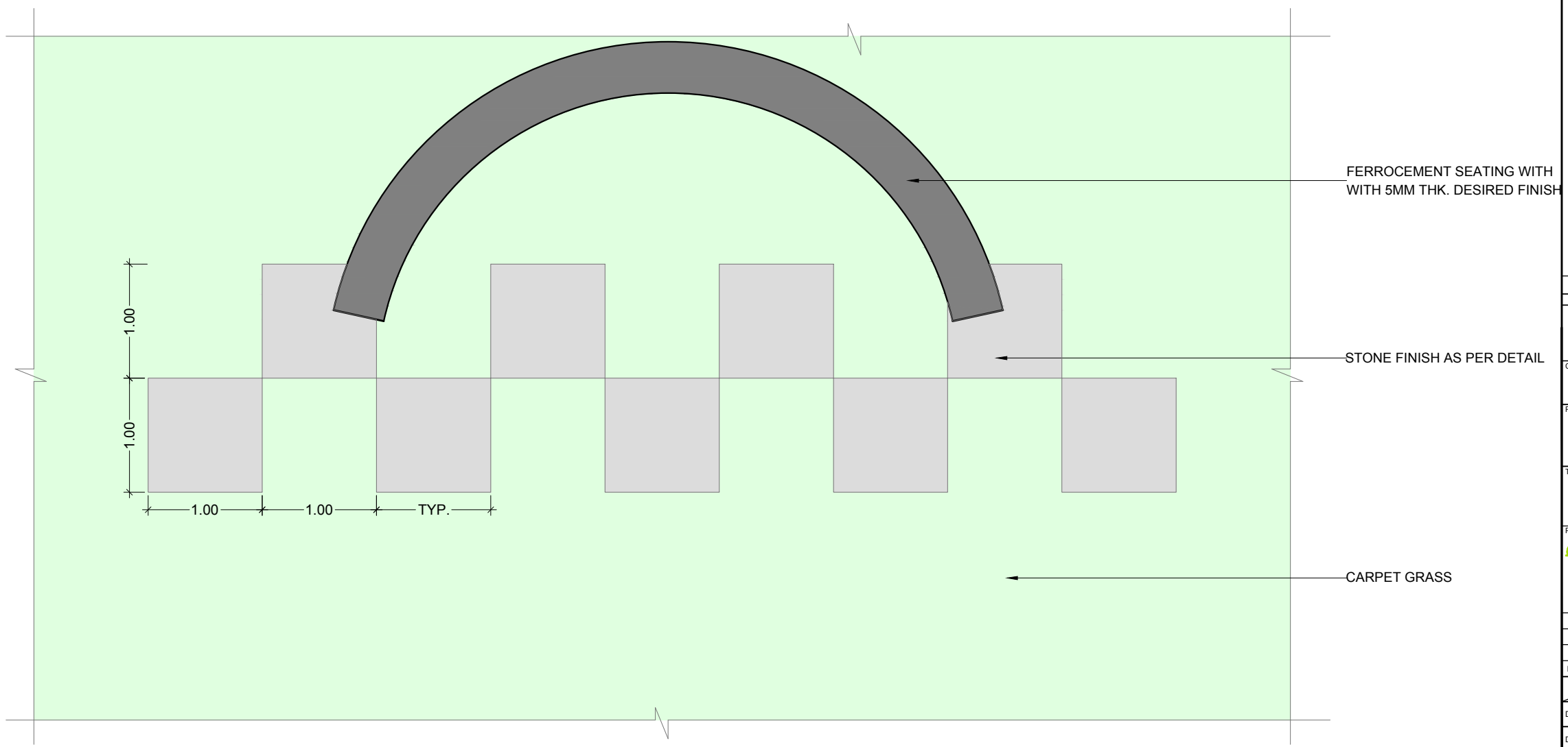
ENLARGE PLAN OF SEATING TYPE -1 (TYP.) (SCALE : 1:50)
