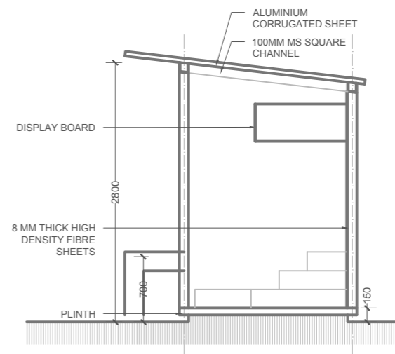
SECTION-1 Scale-1:50
