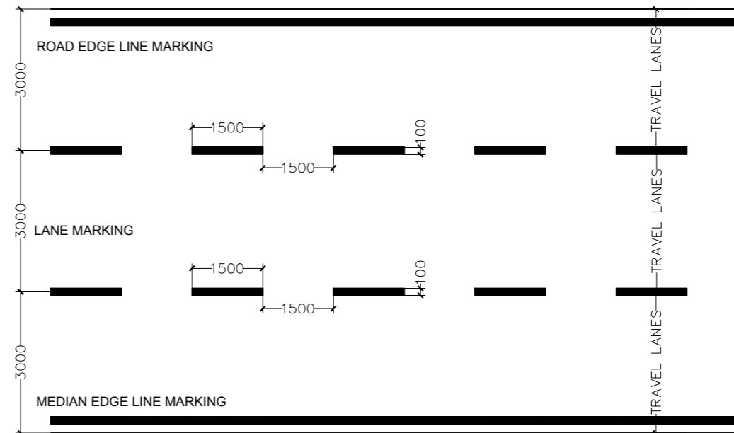
LANE MARKING DETAILS 1:100
