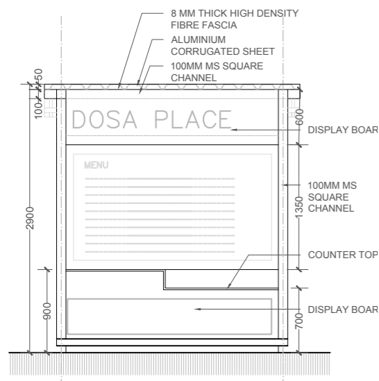
FRONT ELEVATION Scale-1:50
