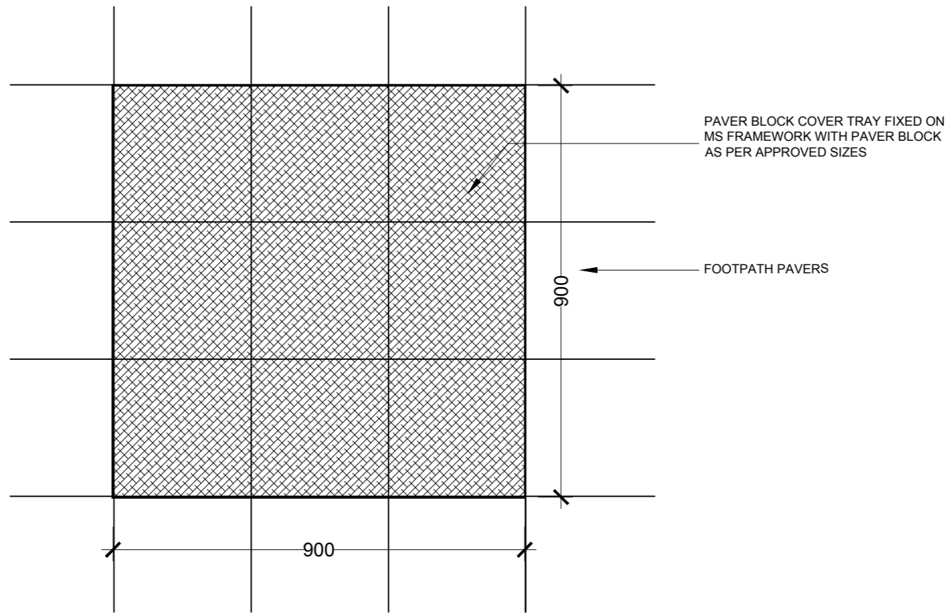
PLAN - CHAMBER COVER SCALE 1:10
