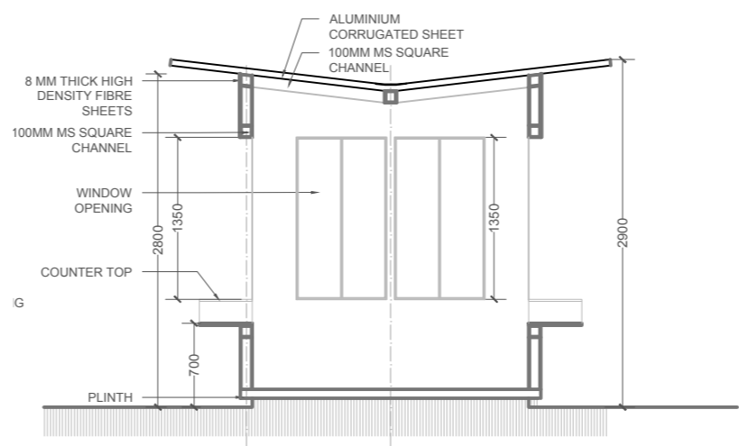
SECTION-1 Scale-1:50
