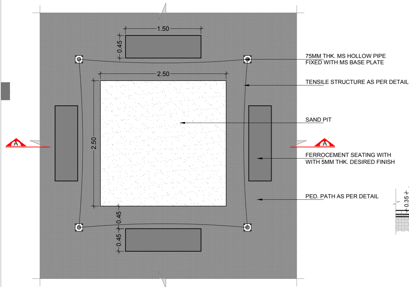
ENLARGE PLAN OF SAND PIT AREA (TYP.) (SCALE : 1:50)
