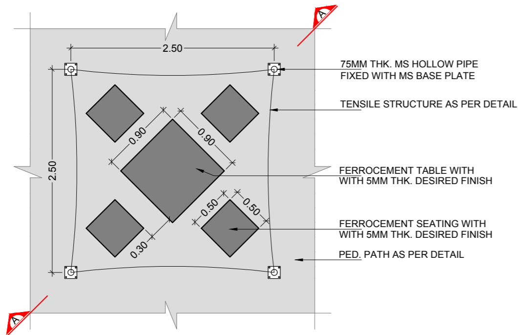
ENLARGE PLAN OF SEATING AREA (TYP.) (SCALE : 1:50)
