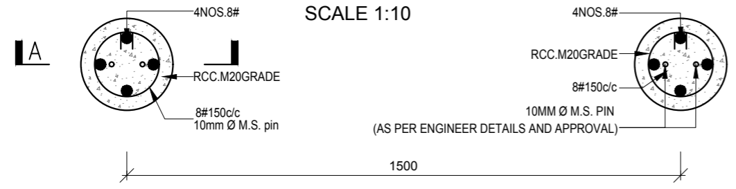
PLAN SCALE 1:10
