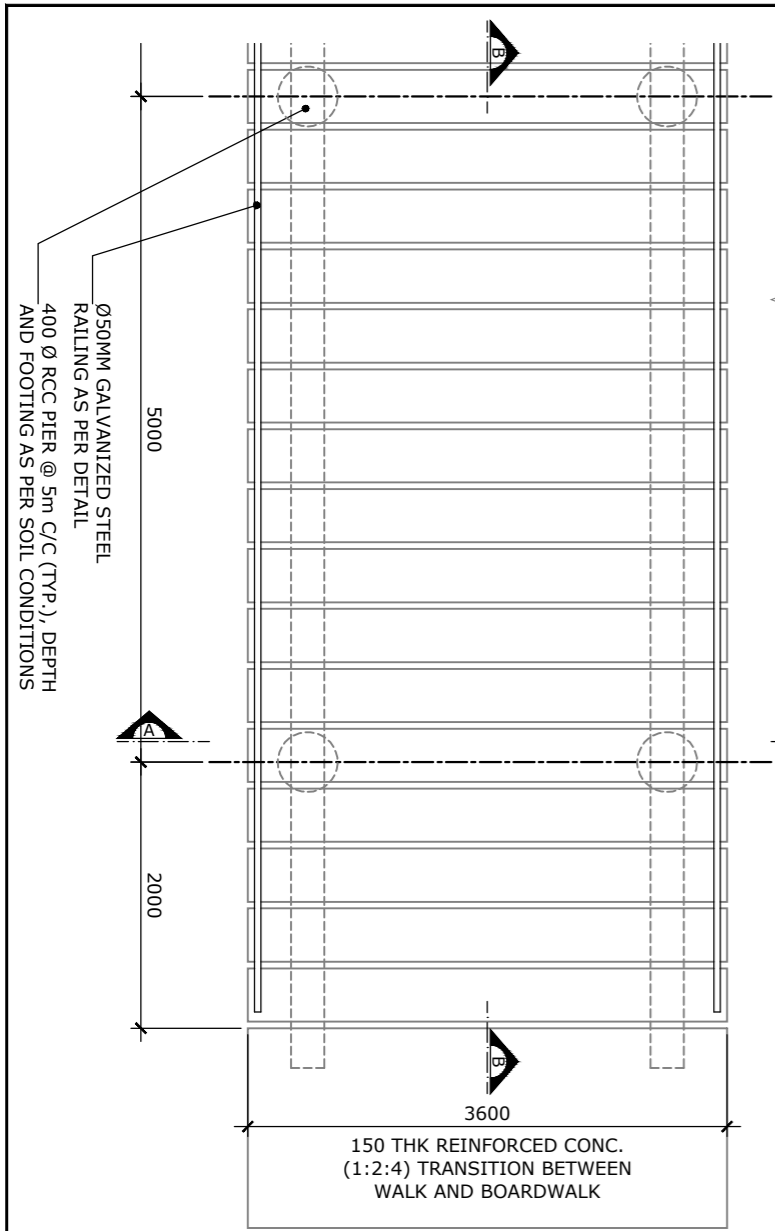
BOARDWALK PLAN SCALE 1:50
