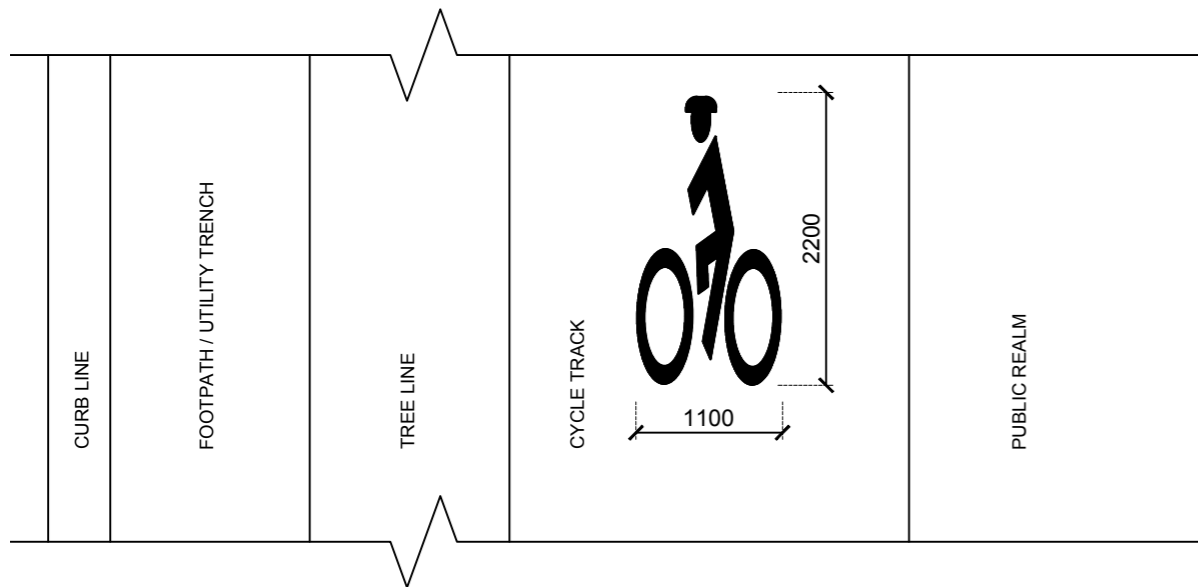
CYCLE TRACK / PEDESTRIAN SYMBOL MARKING 1:50
