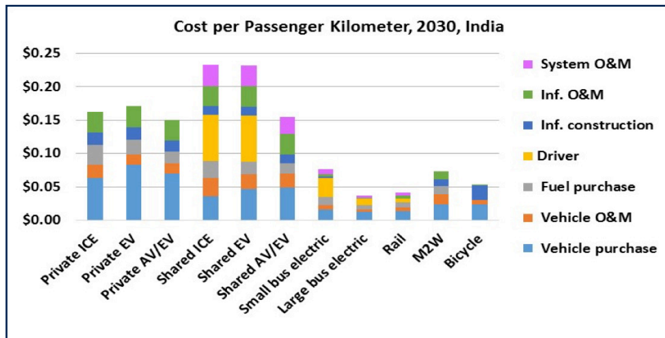
Figure 15. Cost per passenger kilometer by mode, 2030, U.S. and India examples (Note: y axes are not aligned; Indian costs are far lower than U.S. costs)
