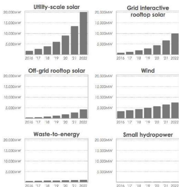
Figure 2: Projected capacity addition to meet the targets, by year and technology type
