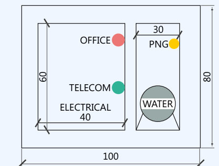
FOR ROADS/STREETS WITHOUT FOOTPATH (DIMENSIONS ARE IN CM)
