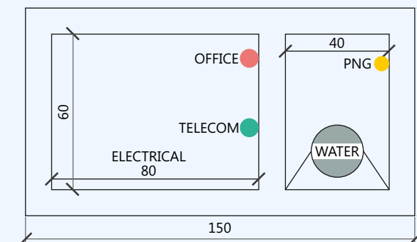
FOR ROADS/STREETS WITH FOOTPATH (DIMENSIONS ARE IN CM)
