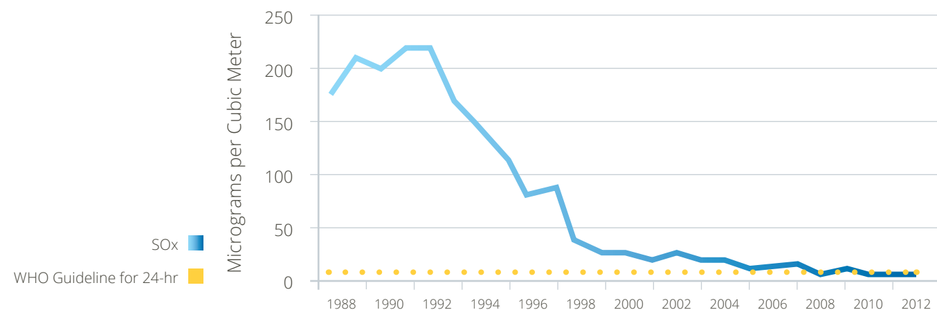
Figure 4: Istanbul Annual Average SO 2 Concentrations 1988-2012
