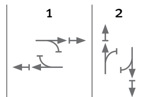
Figure 4.12 The signal phasing plan for a squareabout. Right-turning vehicles enter the queuing spaces during the first phase and exit the ahead of straight-moving traffic during the next phase.
