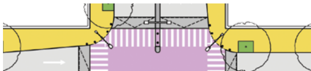
Figure 4.5 The crosswalk is a clear space ahead of the vehicle stop line where pedestrians can cross during the appropriate signal phase. The crosswalk should be aligned with the through movement corridor on the footpath.
