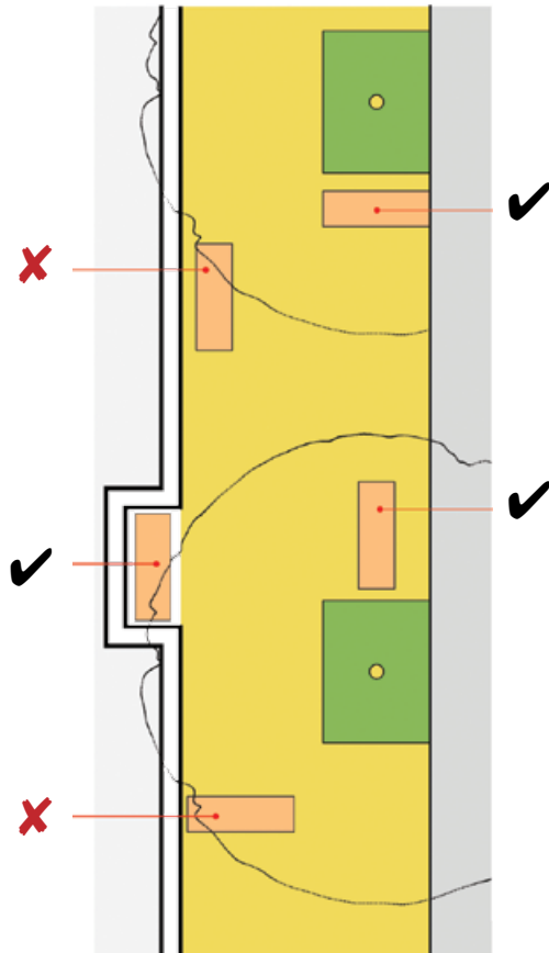
Figure 2.60 Access boxes for underground utilities should not constrain the space needed for through movement. If it is not possible to place utility boxes on private easements, the ideal location is in line with tree pits, to avoid conflicts with pedestrian movements.
