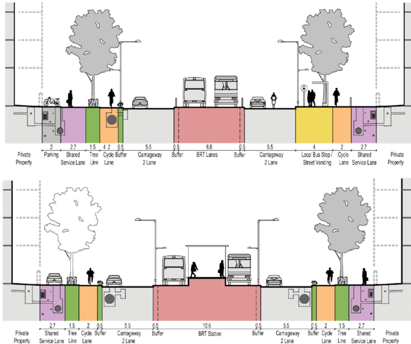
Figure 5.22 The standard section for the 36m street.
