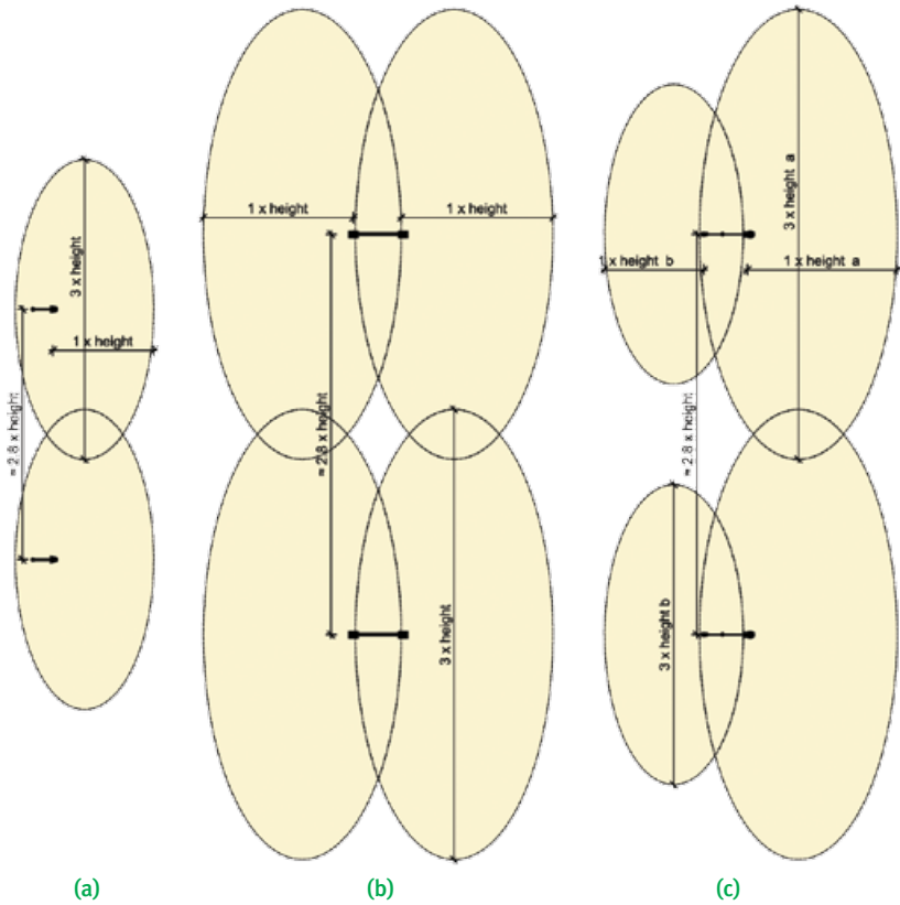
Figure 2.51 Street lights typically illuminate an elliptical area. As a rule of thumb, the longitudinal dimension is equivalent to three times the pole height, and horizontal dimension is slightly longer than the pole height.
