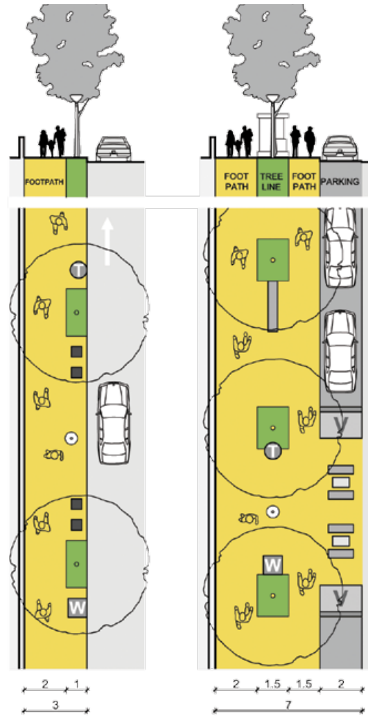
Figure 2.4 The smallest well functioning footpath/tree package has a width of 3 m, including a 2 m clear space and 1 m tree pits. Street furniture is positioned in line with the tree pits to maintain 2 m of clear space.
