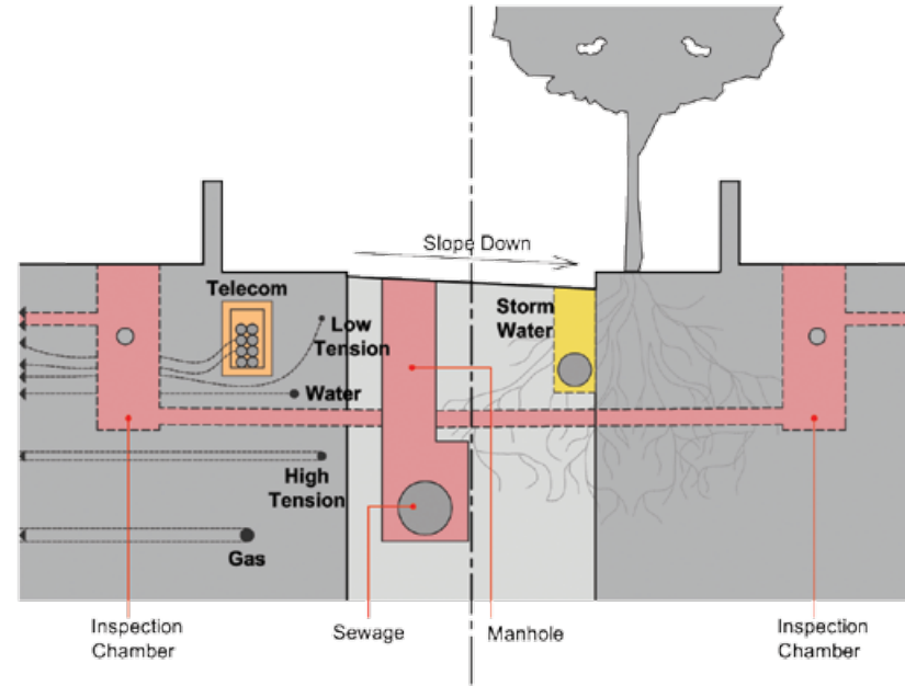
Figure 2.61 The placement of underground utilities should be coordinated with the location of street trees so that the trees are not disturbed if utilities are dug up for maintenance or replacement. Telecommunications, fresh water, and electricity lines generally can be accommodated within a 1.5–2m wide area at the edge of the right-of-way. Sewage and storm water lines are usually placed closer to the centre of the cross section.
