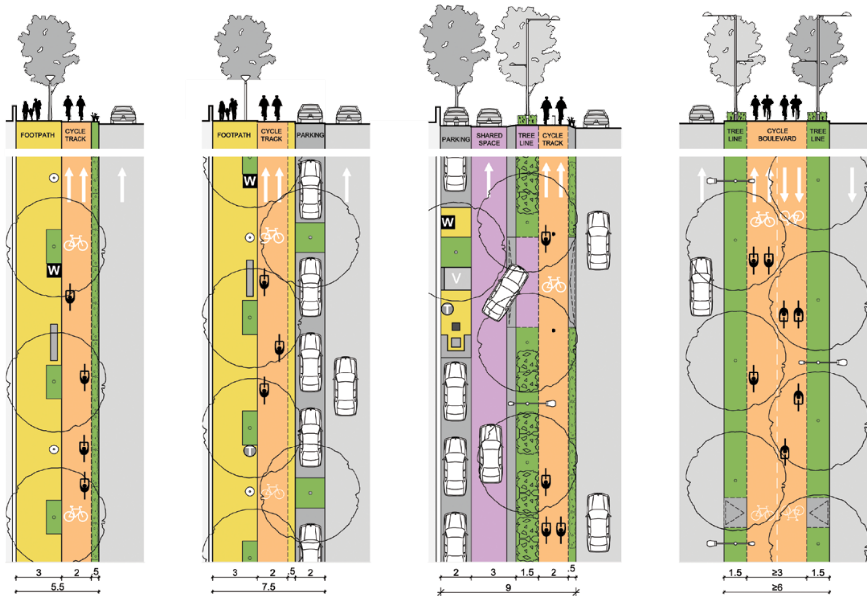
Figure 2.8 A clear width of 2 m is needed for one-way movement of cycles. To accommodate cycle rickshaws a minimum 2.5 m width is recommended, and to accommodate two-way movement, 3 m is recommended. A 0.5 m buffer is needed between a cycle track and motor vehicle or parking lanes. The buffer can accommodate ramps and storm water catch pits. The buffer should be paved if it is adjacent to a parking lane.
