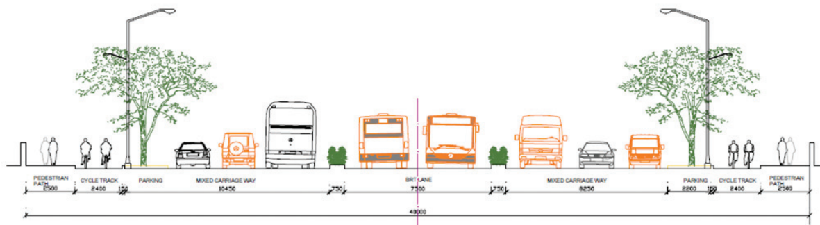
Figure 4.7 Road section proposed at 40 m ROW
