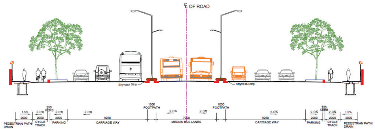
Figure 4.4 Road section at 40 m ROW
