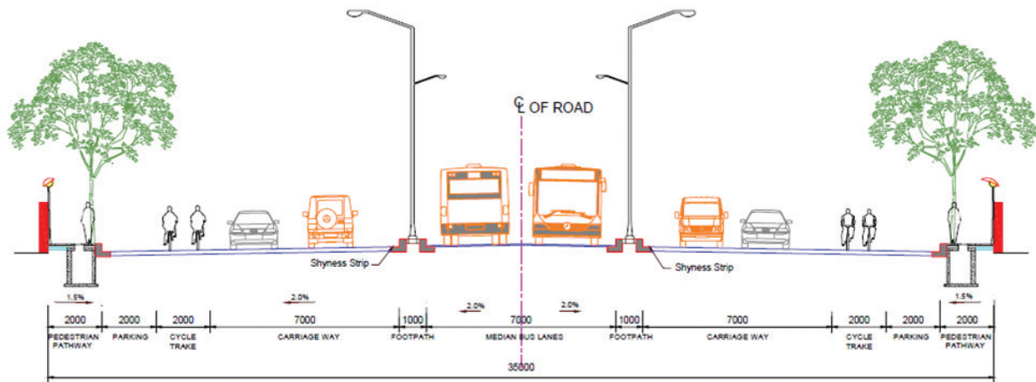
Figure 4.5 Road section proposed at 35 m ROW
