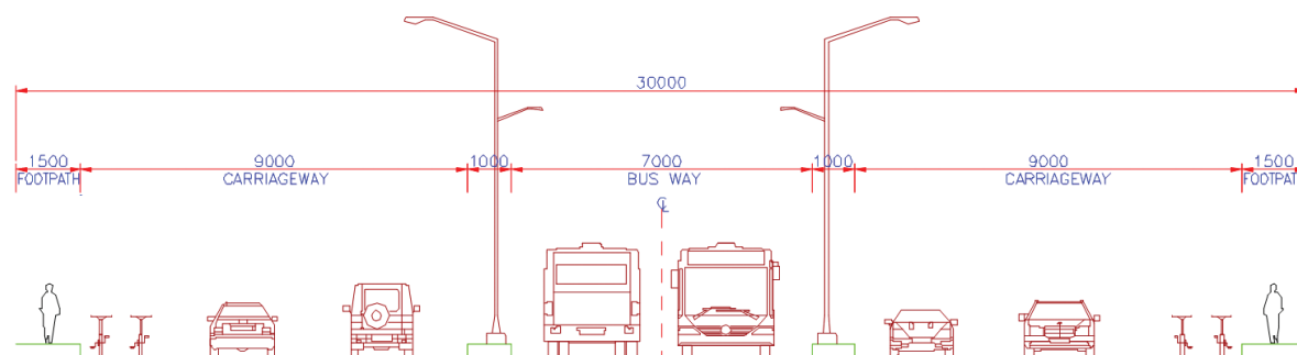
Figure 3.33 Road section at 30 m ROW
