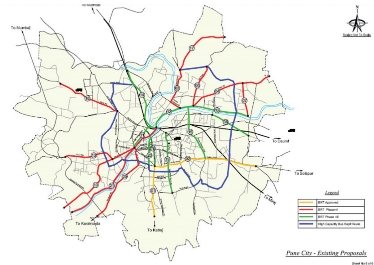
Figure 3.22 Existing BRT proposals in Pune
