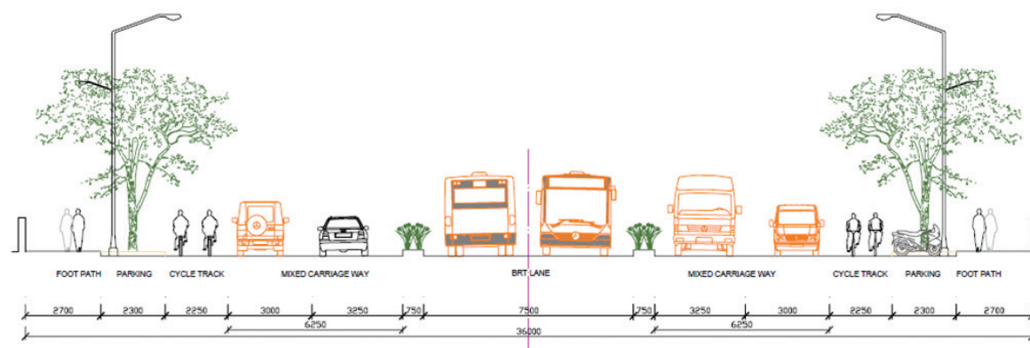
Figure 4.8 Road section proposed at 35 m ROW
