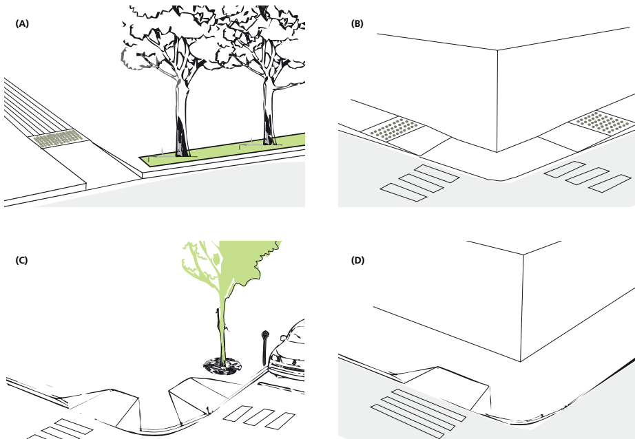
FIGURE 8: EXAMPLES OF CURB RAMPS
