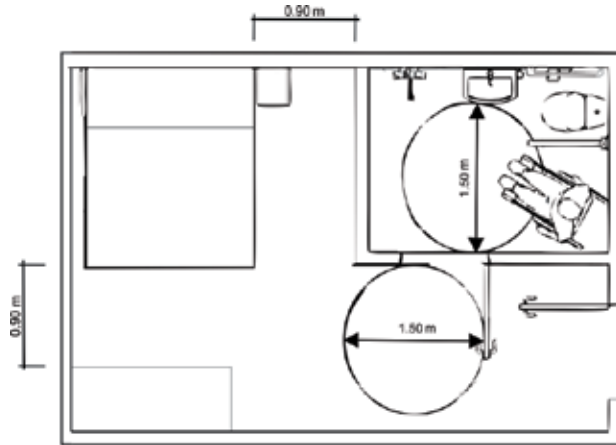
FIGURE 23: BEDROOM WITH BATHROOM
