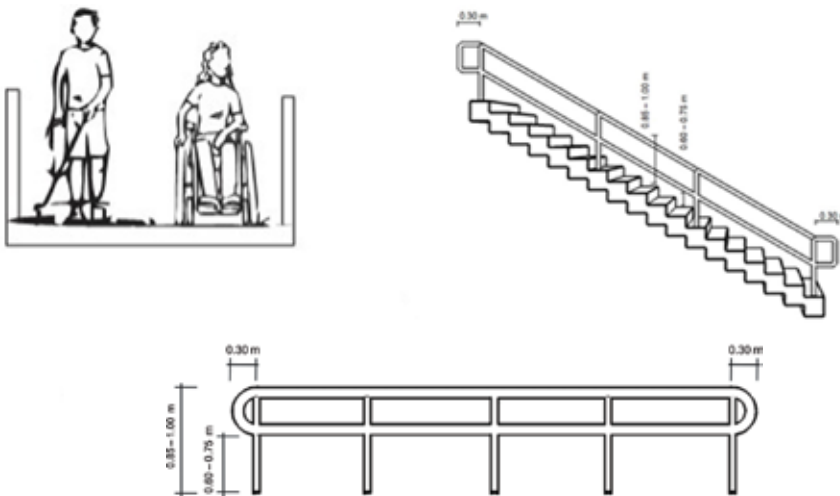
FIGURE 19: RAILINGS AND HANDRAILS
