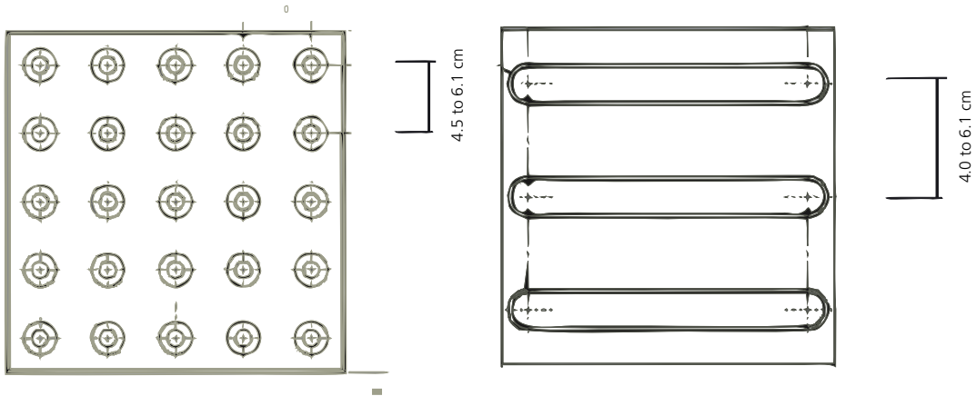
FIGURE 6: TACTILE WARNING AND DIRECTIONAL FLOOR
