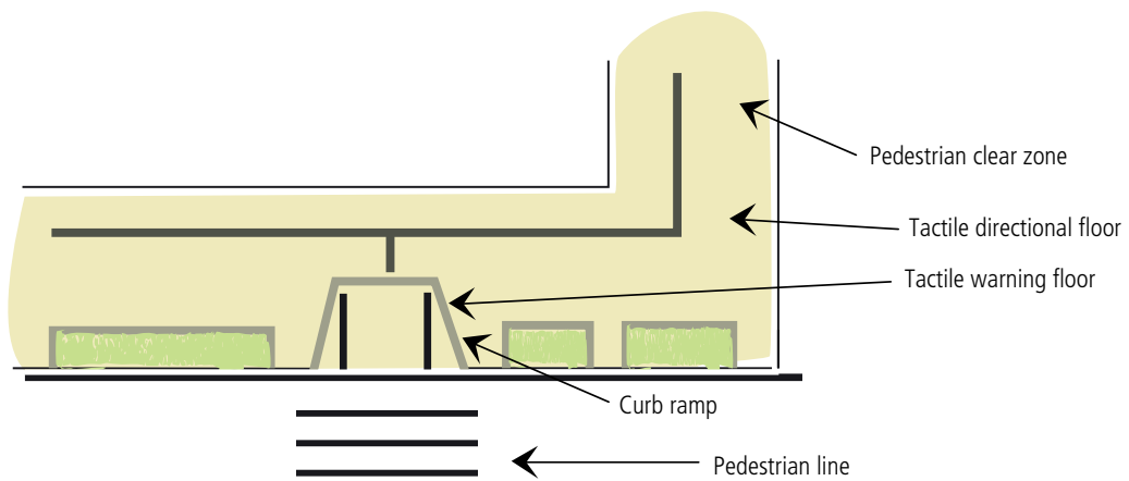
FIGURE 12: KEY ELEMENTS OF AN ACCESSIBLE ROUTE
