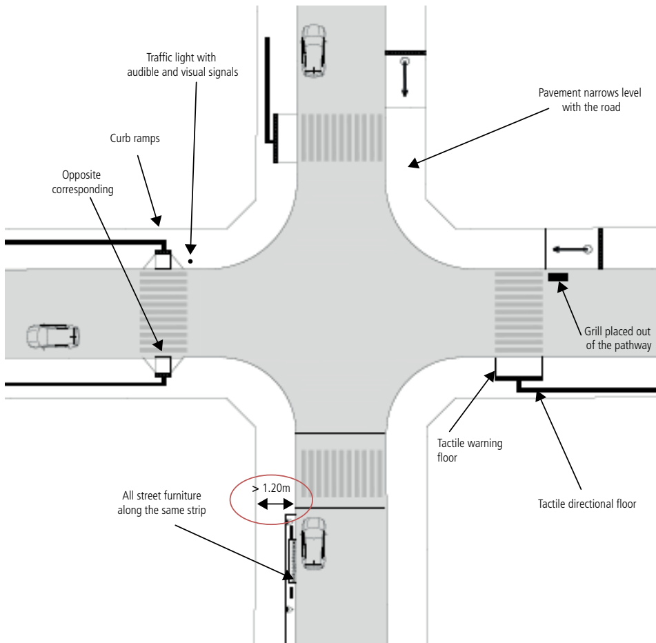
FIGURE 30: ACCESSIBLE ROUTES AND PEDESTRIAN CROSSINGS
