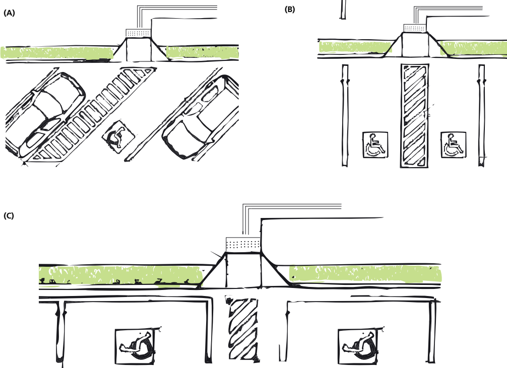
FIGURE 11: PARKING SPACES
