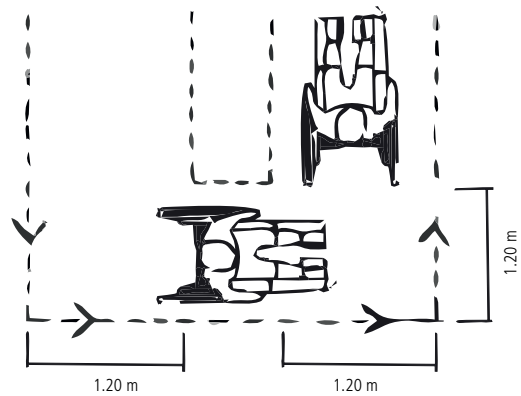
FIGURE 22: TURNING SPACE IN CORRIDORS
