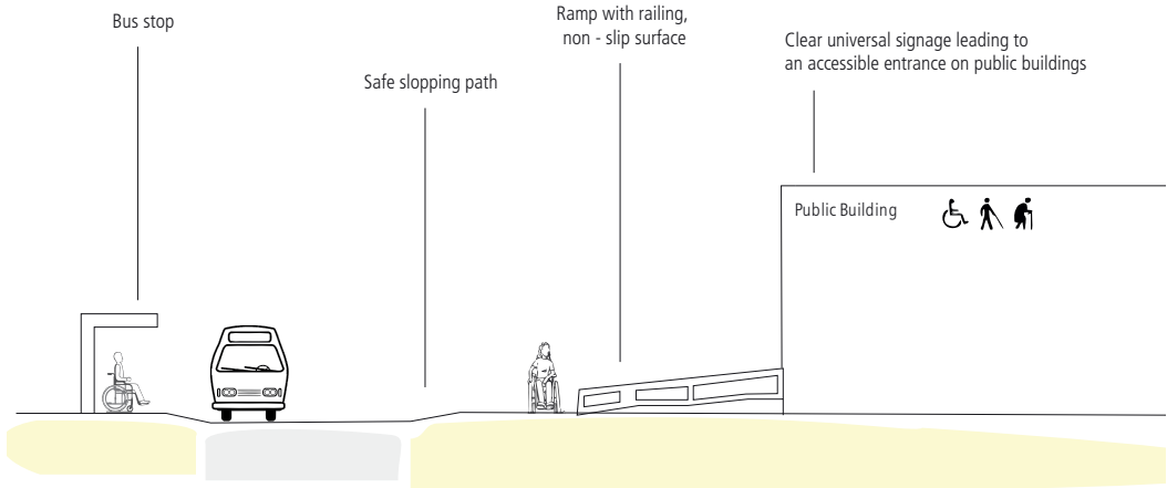
FIGURE 13: ACCESSIBLE ROUTE
