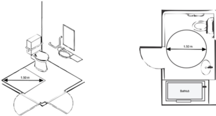
FIGURE 26: RESTROOMS WITH CLEAR CIRCUMSCRIBED MANOEUVRING AREA
