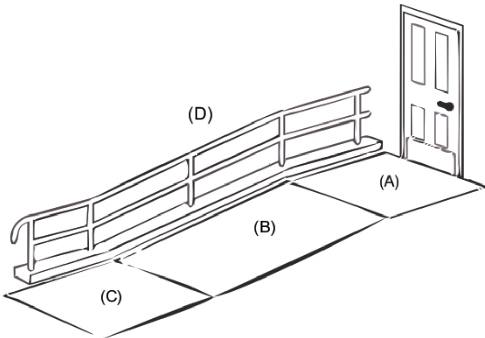
FIGURE 15: RAMPED ACCESS
