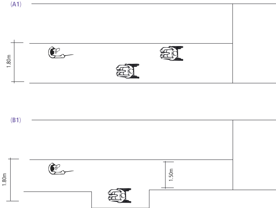
FIGURE 16: RAMPS FOR CONSTANT (A1) AND FREQUENT (B1) TWO-WAY TRAFFIC
