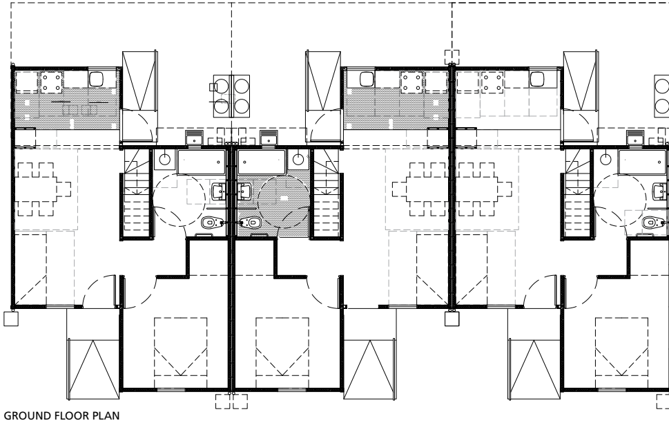
FIGURE 52: GROUND FLOOR PLAN-ADAPTED UNITS WITH ACCESSIBLE GROUND FLOOR
