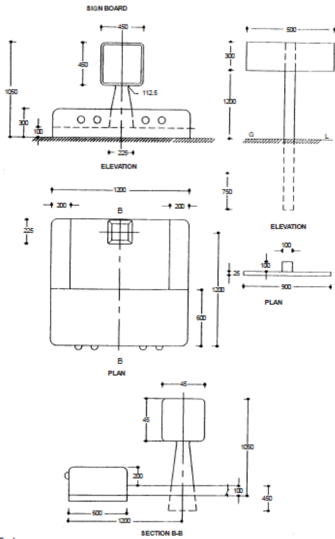
Fig. 16.3 : Sign/Name Board
