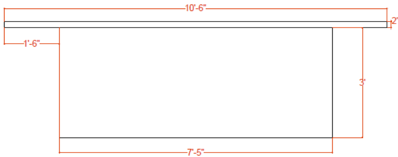
FRONT ELEVATION OF TABLE
